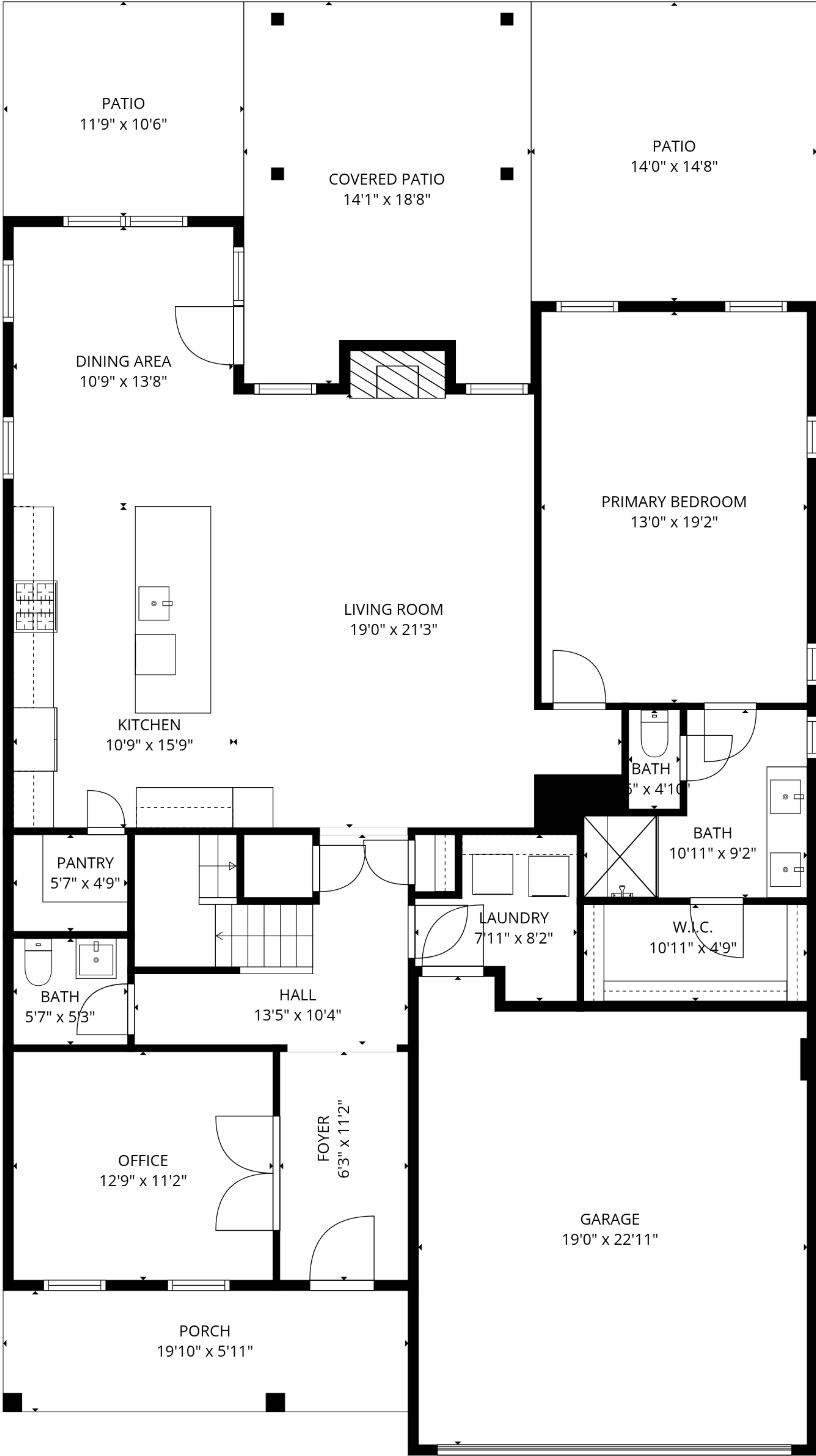
1st floor
